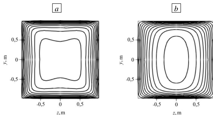
Fig. 5. The velocity isolines in the duct cross section: calculation be means of the EOF library (a, b), analytical solution [32] (c, d); the walls have infinite electrical conductivity (a, c), isolated walls (b, d)
